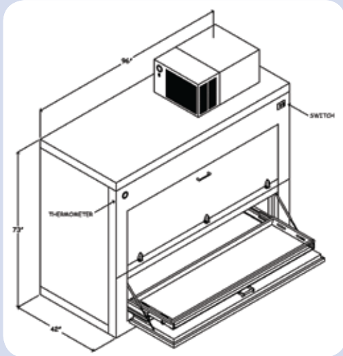
CAT NO. 90-0962 TWO BODY
