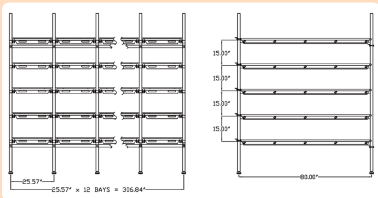
DIAGRAM of Mortuary Storage Rack System CAT No. 90-1030
