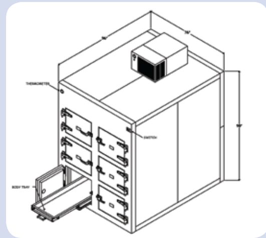
CAT NO. 90-0942 Six Body Vertical
