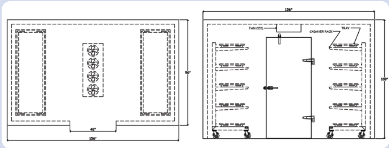
DESIGN for (2) CADAVER RACKS 8 - 10 BODY STORAGE
