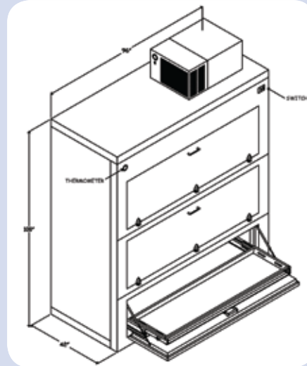
CAT NO. 90-0964 THREE BODY
